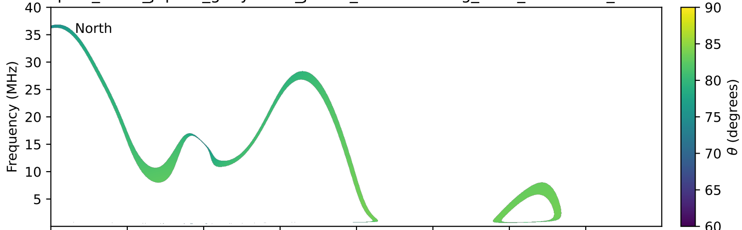
expres_earth_jupiter_ganymede_jrm33_lossc-wid1deg_3kev_20180928_v11.cdf
