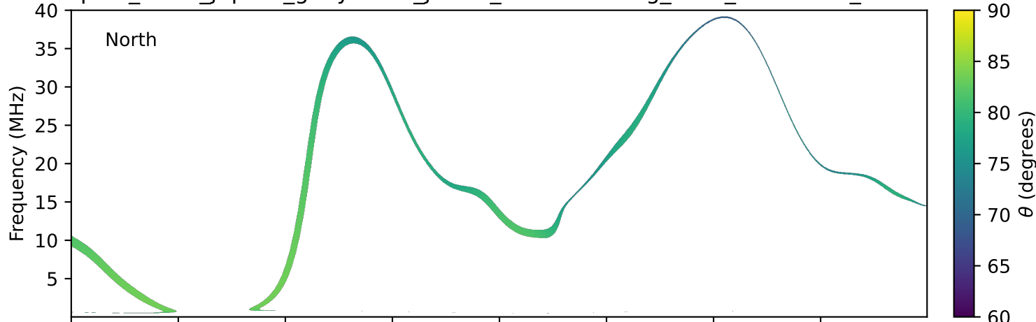
expres_earth_jupiter_ganymede_jrm33_lossc-wid1deg_3kev_20180904_v11.cdf
