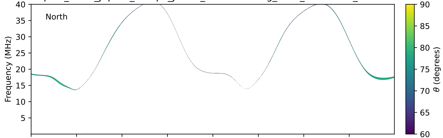
expres_earth_jupiter_europa_jrm33_lossc-wid1deg_3kev_20180921_v11.cdf
