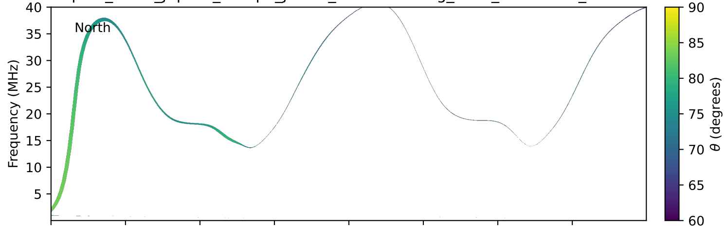
expres_earth_jupiter_europa_jrm33_lossc-wid1deg_3kev_20180903_v11.cdf
