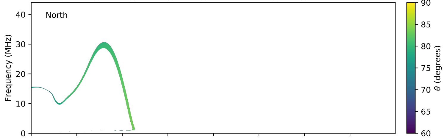
expres_earth_jupiter_europa_jrm09_lossc-wid1deg_3kev_20180922_v01.cdf
