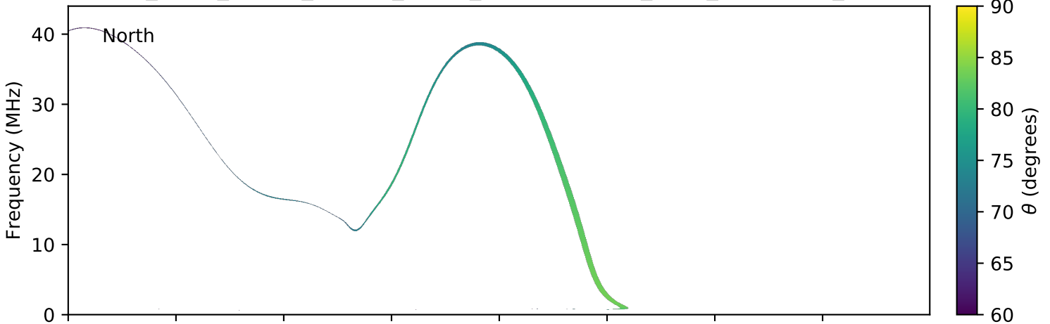
expres_earth_jupiter_europa_jrm09_lossc-wid1deg_3kev_20180918_v01.cdf
