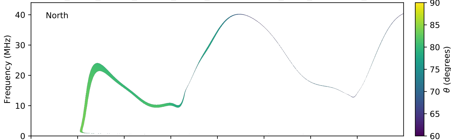
expres_earth_jupiter_europa_jrm09_lossc-wid1deg_3kev_20180917_v01.cdf
