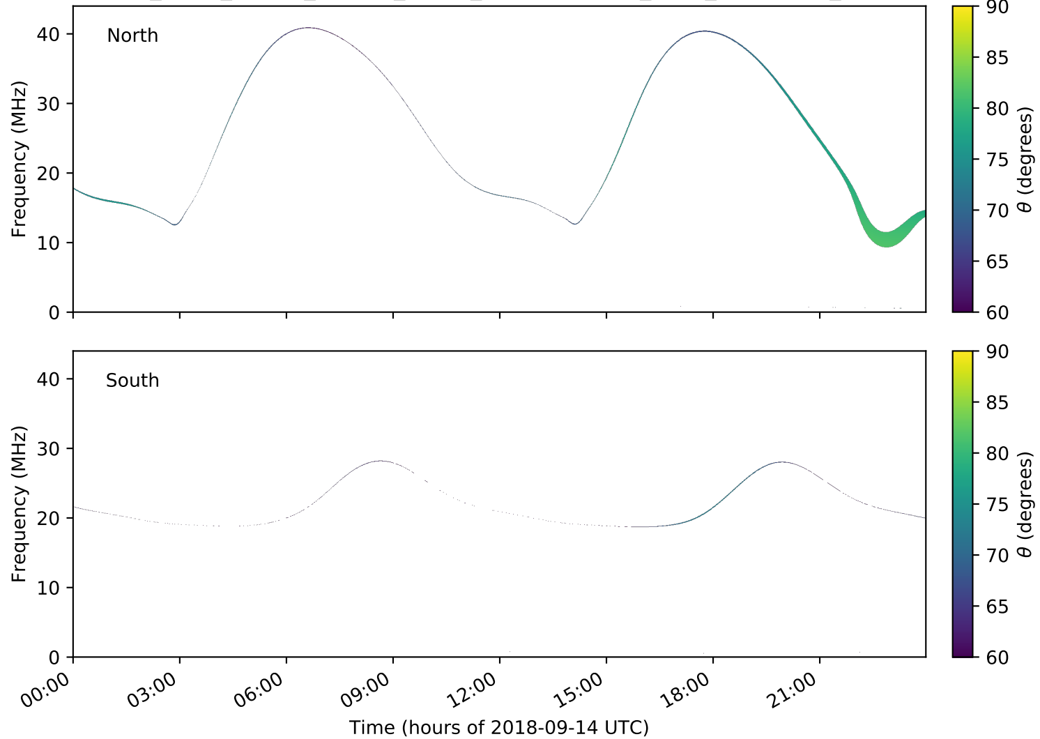
expres_earth_jupiter_europa_jrm09_lossc-wid1deg_3kev_20180914_v01.cdf
