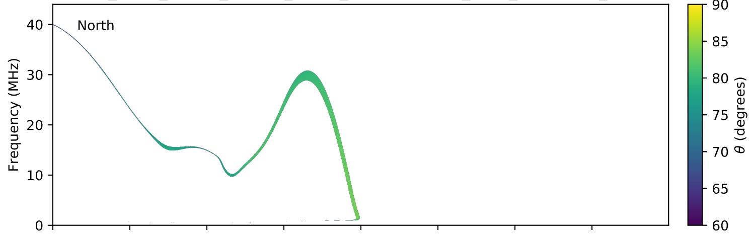
expres_earth_jupiter_europa_jrm09_lossc-wid1deg_3kev_20180904_v01.cdf
