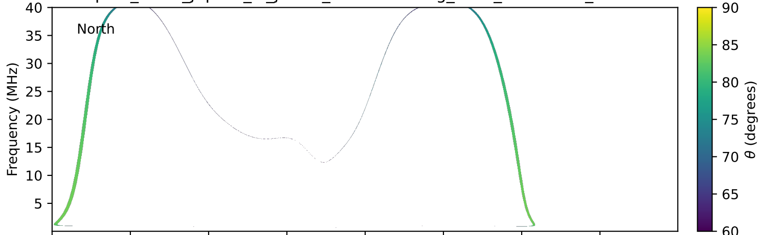
expres_earth_jupiter_io_jrm33_lossc-wid1deg_3kev_20180829_v11.cdf
