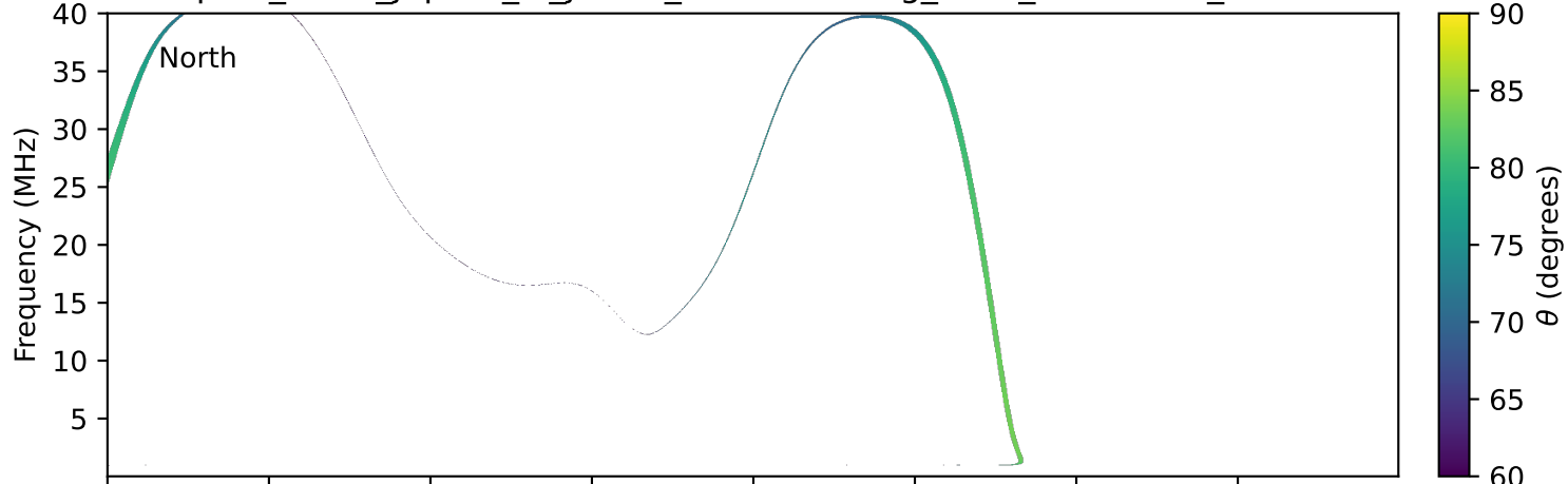
expres_earth_jupiter_io_jrm33_lossc-wid1deg_3kev_20180822_v11.cdf
