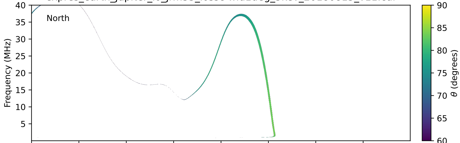
expres_earth_jupiter_io_jrm33_lossc-wid1deg_3kev_20180815_v11.cdf
