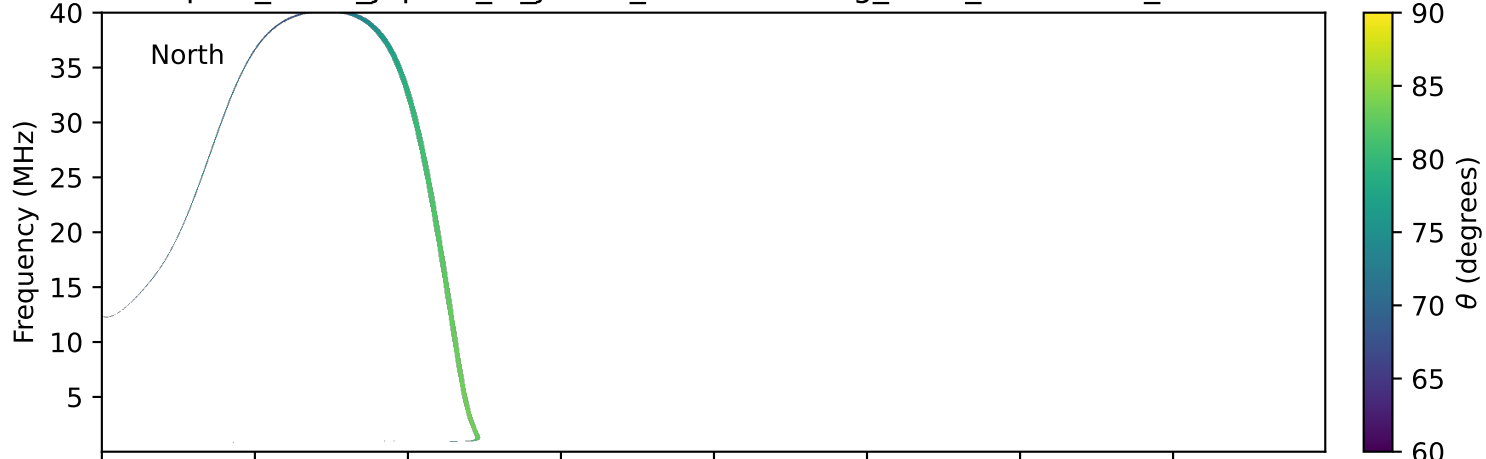
expres_earth_jupiter_io_jrm33_lossc-wid1deg_3kev_20180810_v11.cdf
