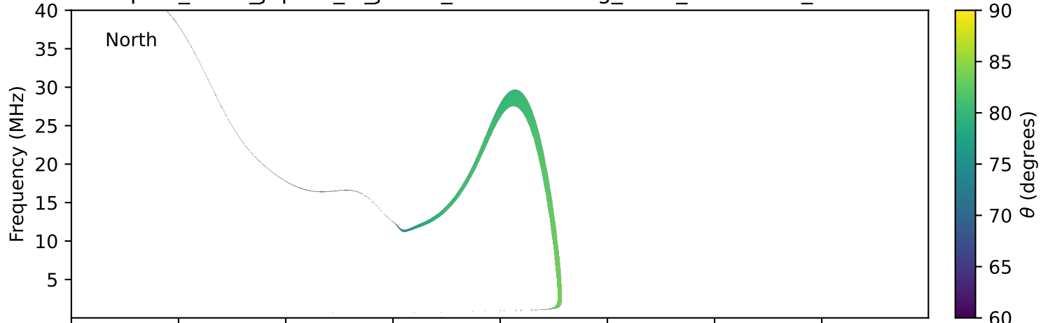
expres_earth_jupiter_io_jrm33_lossc-wid1deg_3kev_20180808_v11.cdf
