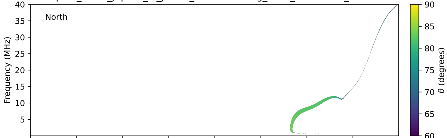
expres_earth_jupiter_io_jrm33_lossc-wid1deg_3kev_20180807_v11.cdf
