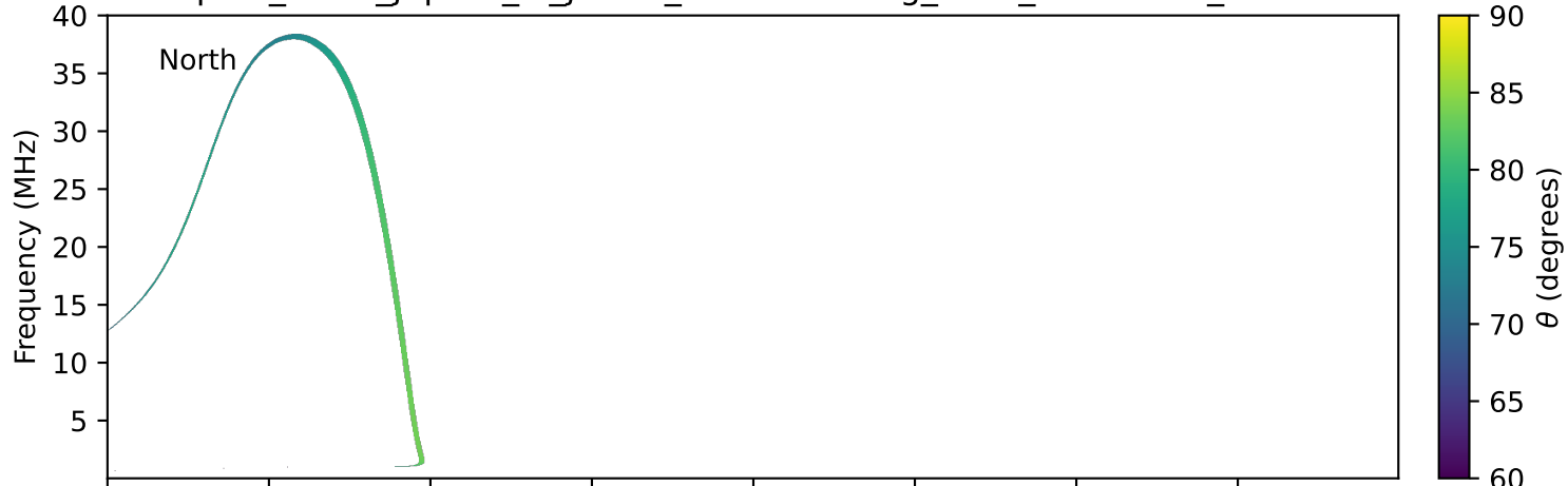
expres_earth_jupiter_io_jrm33_lossc-wid1deg_3kev_20180803_v11.cdf
