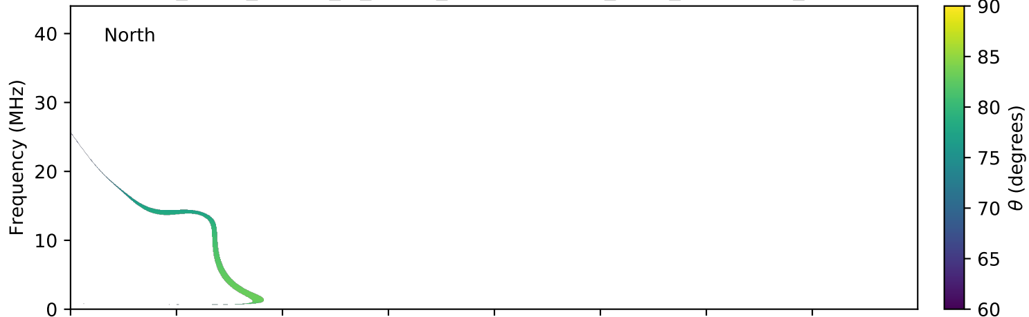
expres_earth_jupiter_io_jrm09_lossc-wid1deg_3kev_20180826_v01.cdf
