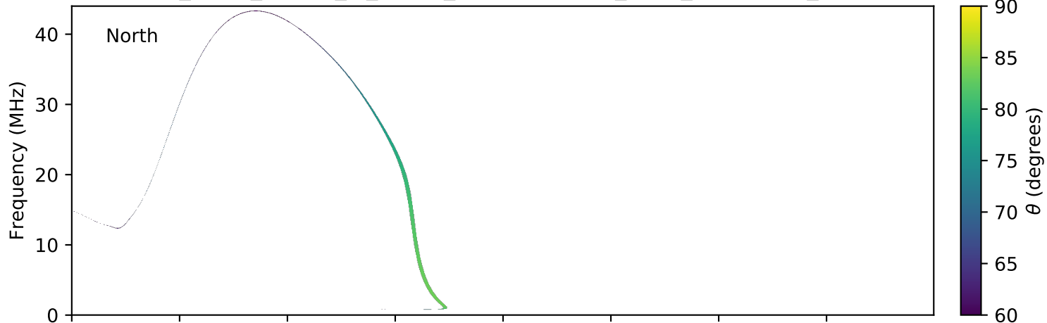
expres_earth_jupiter_io_jrm09_lossc-wid1deg_3kev_20180824_v01.cdf
