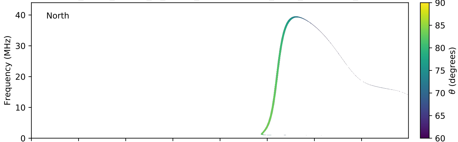
expres_earth_jupiter_io_jrm09_lossc-wid1deg_3kev_20180816_v01.cdf
