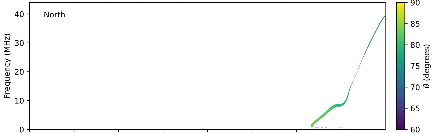
expres_earth_jupiter_io_jrm09_lossc-wid1deg_3kev_20180814_v01.cdf
