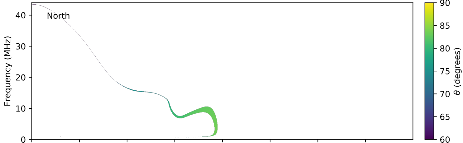
expres_earth_jupiter_io_jrm09_lossc-wid1deg_3kev_20180801_v01.cdf
