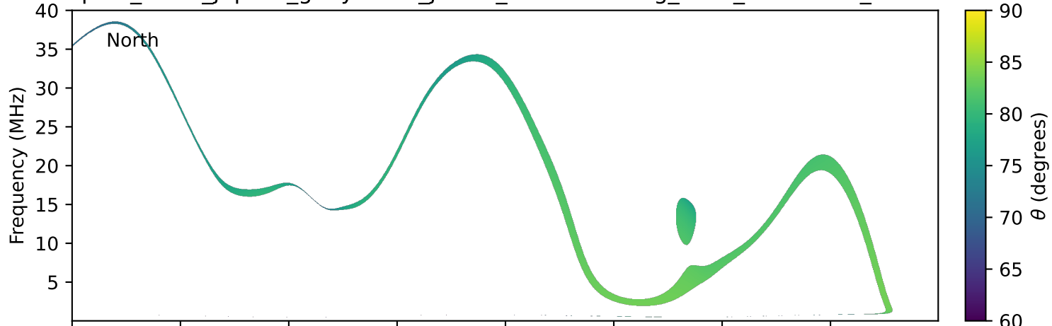
expres_earth_jupiter_ganymede_jrm33_lossc-wid1deg_3kev_20180830_v11.cdf
