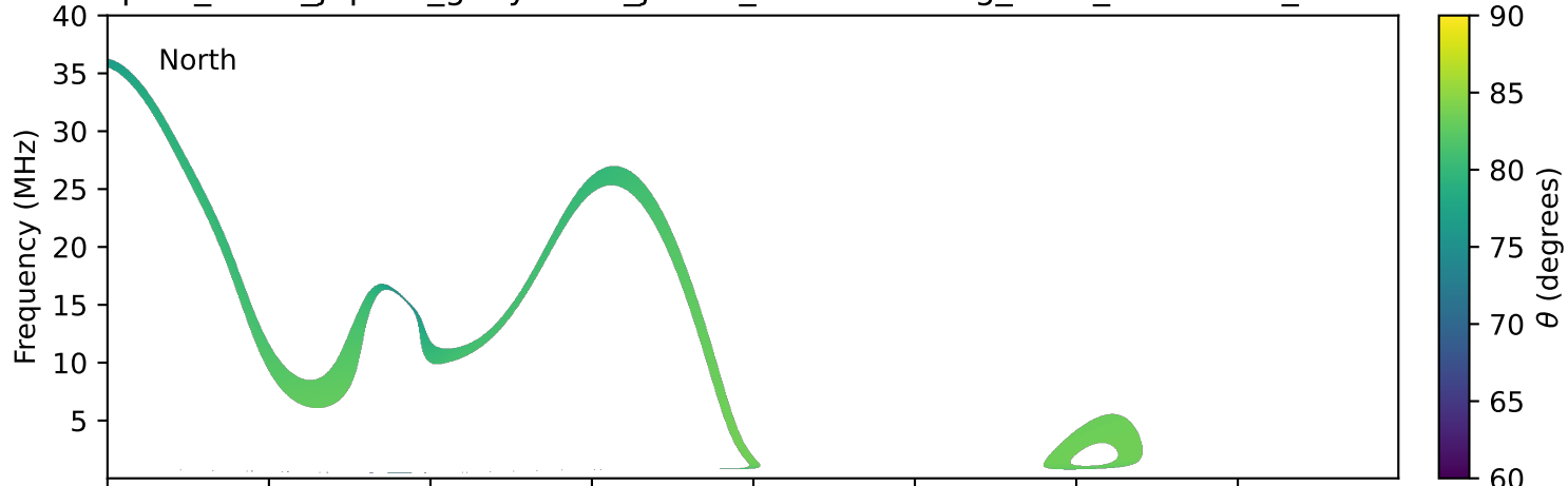
expres_earth_jupiter_ganymede_jrm33_lossc-wid1deg_3kev_20180816_v11.cdf
