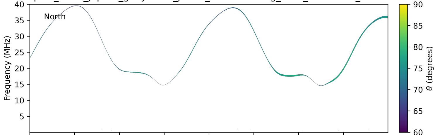
expres_earth_jupiter_ganymede_jrm33_lossc-wid1deg_3kev_20180815_v11.cdf
