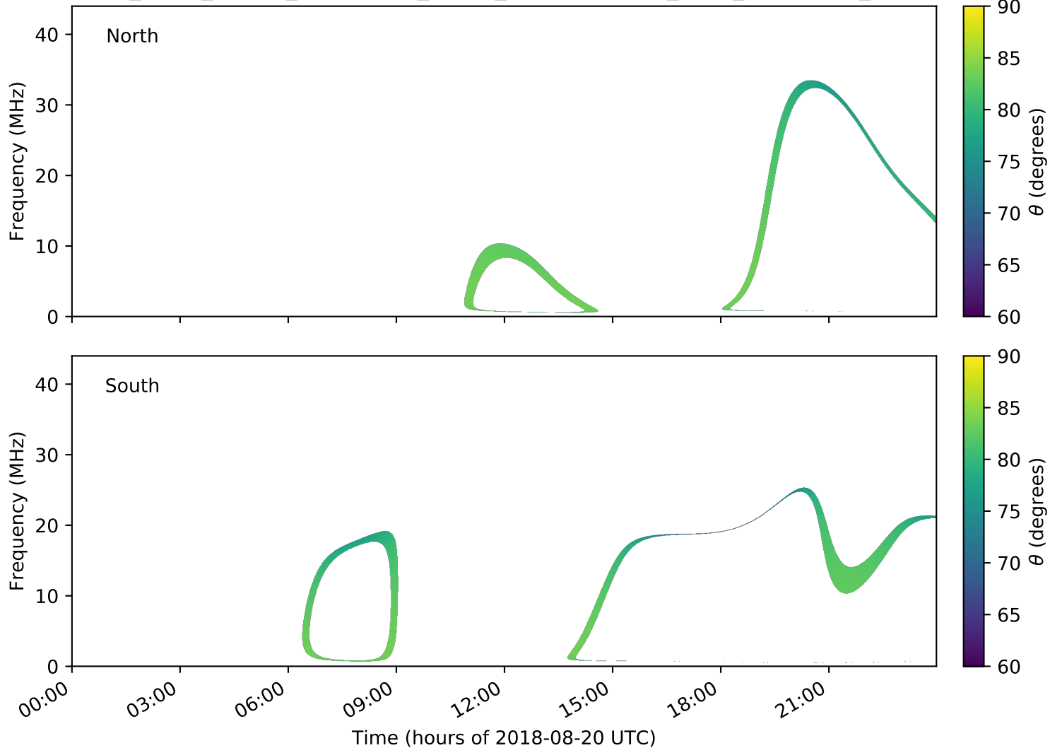
expres_earth_jupiter_ganymede_jrm09_lossc-wid1deg_3kev_20180820_v01.cdf
