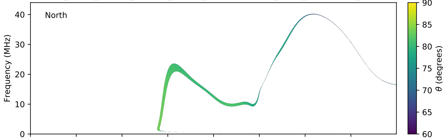
expres_earth_jupiter_europa_jrm09_lossc-wid1deg_3kev_20180830_v01.cdf
