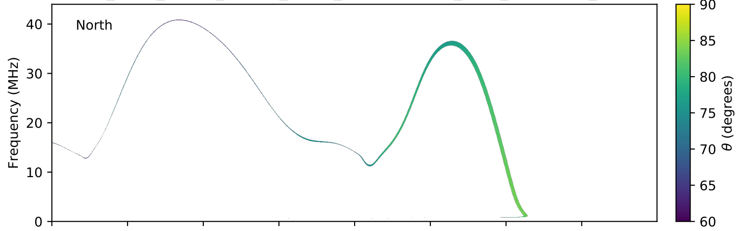
expres_earth_jupiter_europa_jrm09_lossc-wid1deg_3kev_20180824_v01.cdf
