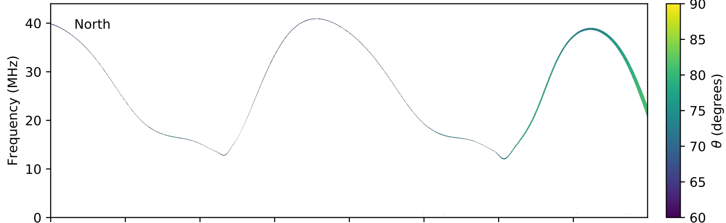
expres_earth_jupiter_europa_jrm09_lossc-wid1deg_3kev_20180813_v01.cdf
