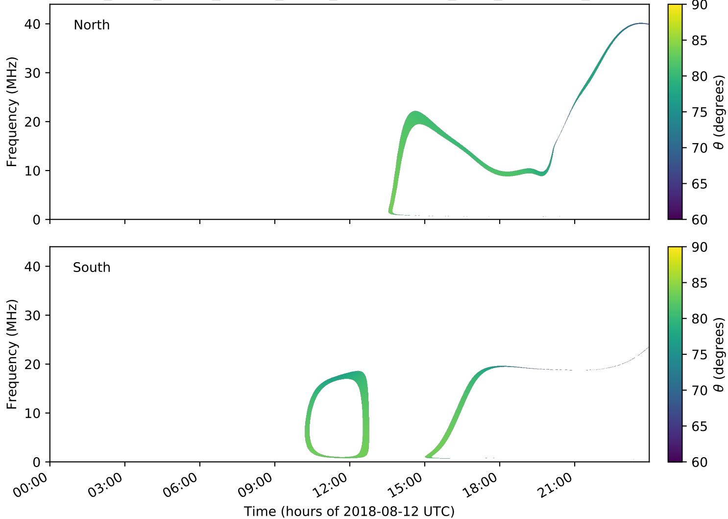
expres_earth_jupiter_europa_jrm09_lossc-wid1deg_3kev_20180812_v01.cdf
