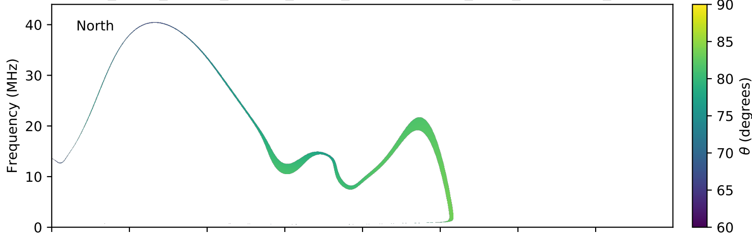
expres_earth_jupiter_europa_jrm09_lossc-wid1deg_3kev_20180810_v01.cdf
