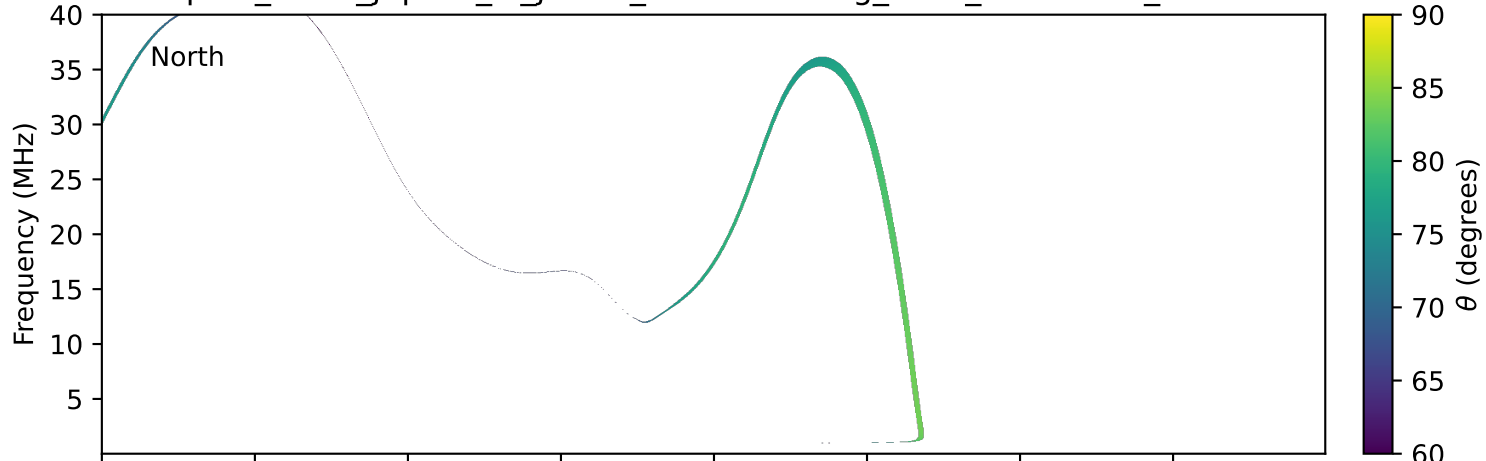
expres_earth_jupiter_io_jrm33_lossc-wid1deg_3kev_20180422_v11.cdf
