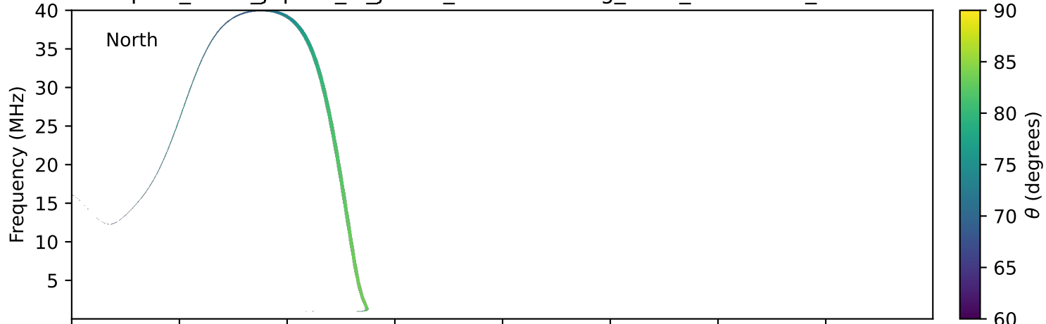
expres_earth_jupiter_io_jrm33_lossc-wid1deg_3kev_20180417_v11.cdf
