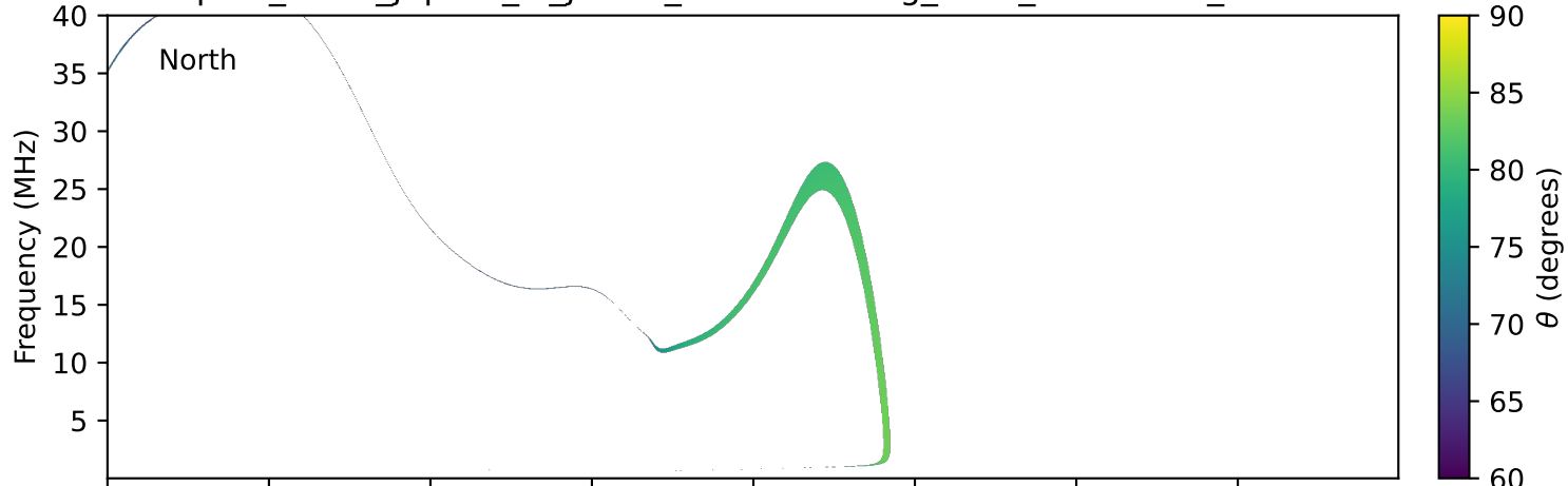
expres_earth_jupiter_io_jrm33_lossc-wid1deg_3kev_20180415_v11.cdf
