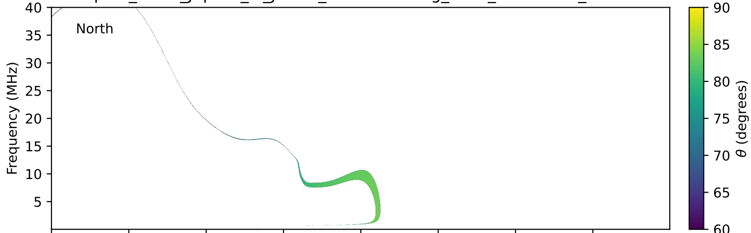
expres_earth_jupiter_io_jrm33_lossc-wid1deg_3kev_20180408_v11.cdf
