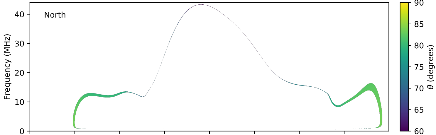
expres_earth_jupiter_io_jrm09_lossc-wid1deg_3kev_20180427_v01.cdf
