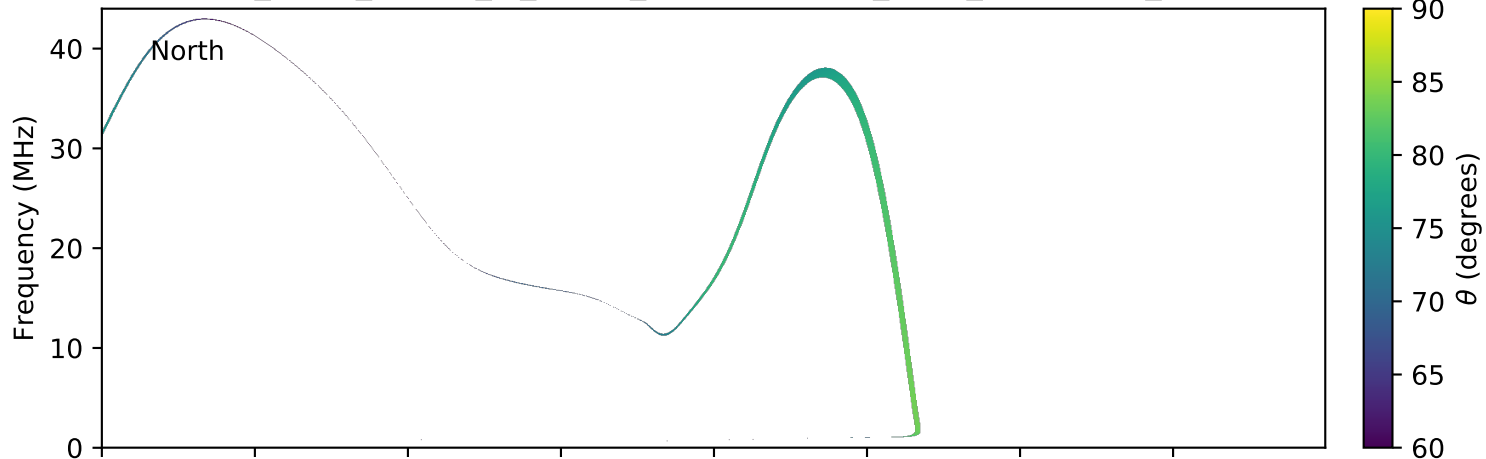
expres_earth_jupiter_io_jrm09_lossc-wid1deg_3kev_20180422_v01.cdf
