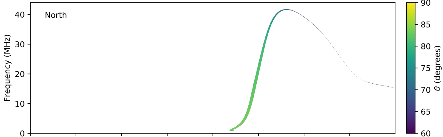
expres_earth_jupiter_io_jrm09_lossc-wid1deg_3kev_20180416_v01.cdf
