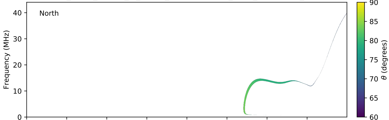
expres_earth_jupiter_io_jrm09_lossc-wid1deg_3kev_20180407_v01.cdf
