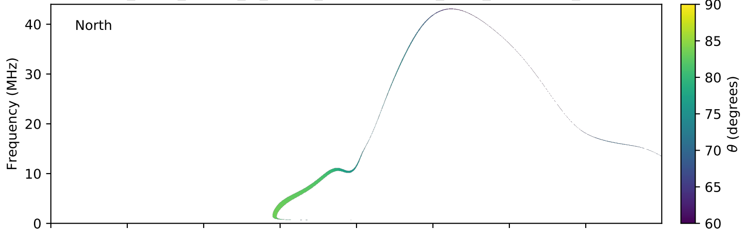
expres_earth_jupiter_io_jrm09_lossc-wid1deg_3kev_20180402_v01.cdf
