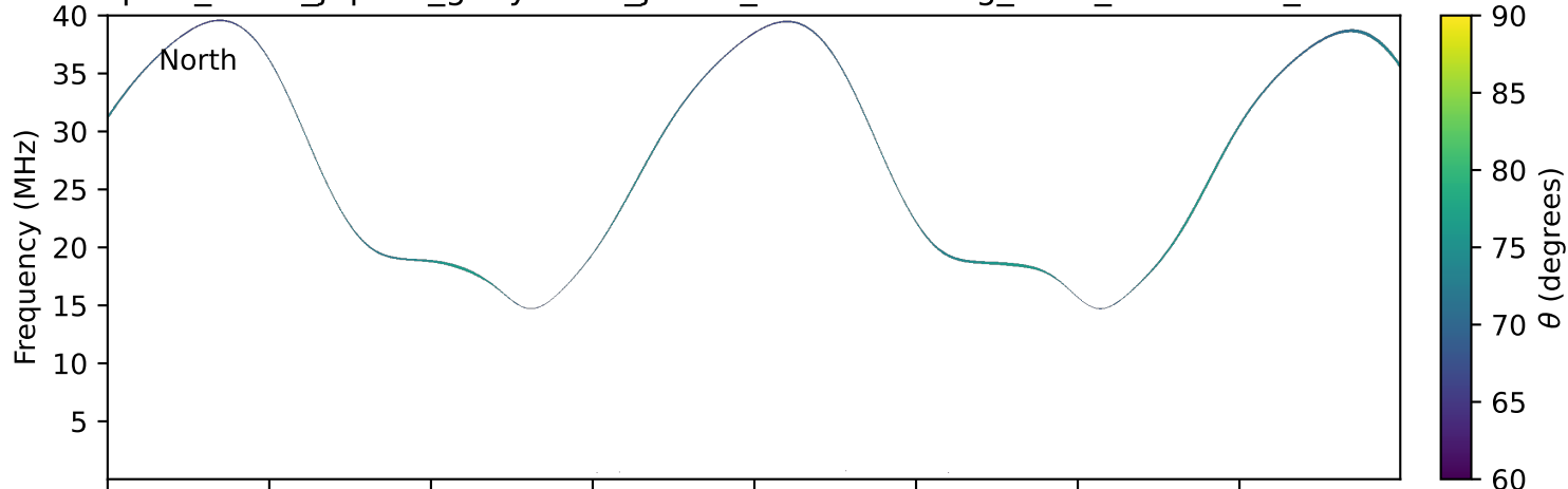
expres_earth_jupiter_ganymede_jrm33_lossc-wid1deg_3kev_20180408_v11.cdf
