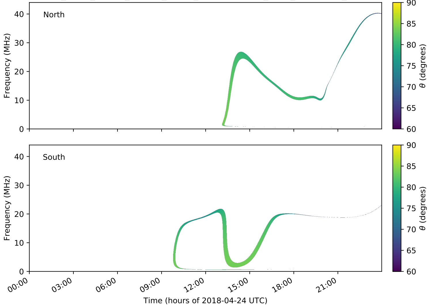
expres_earth_jupiter_europa_jrm09_lossc-wid1deg_3kev_20180424_v01.cdf
