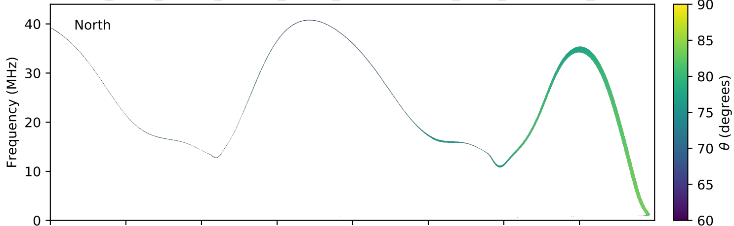
expres_earth_jupiter_europa_jrm09_lossc-wid1deg_3kev_20180418_v01.cdf
