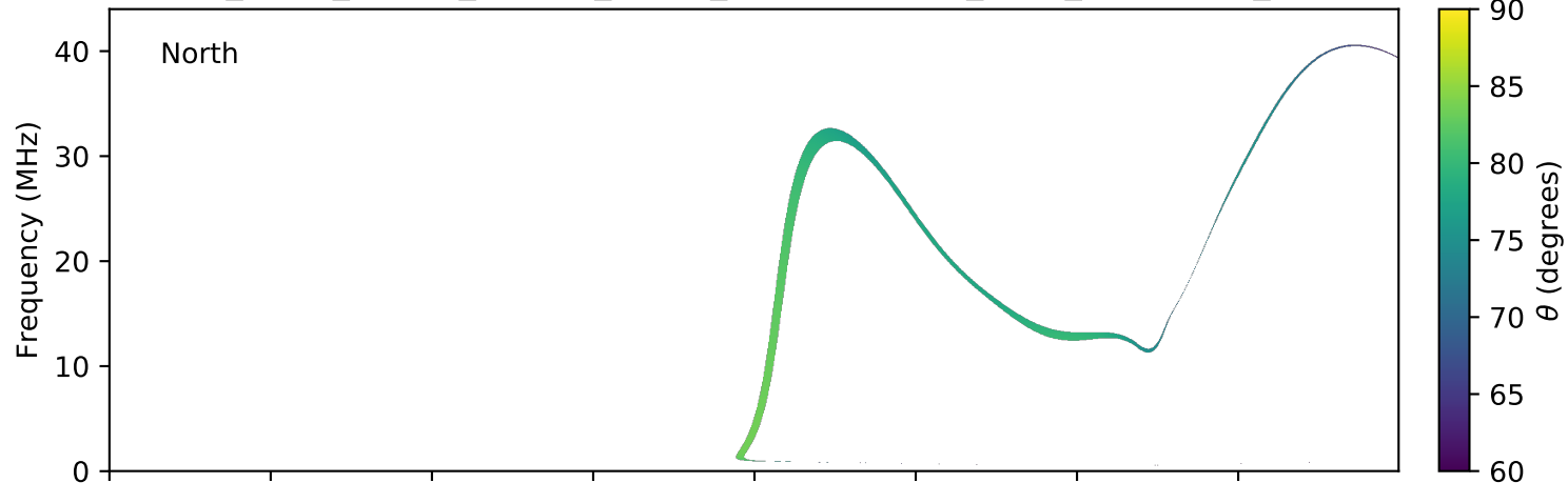
expres_earth_jupiter_europa_jrm09_lossc-wid1deg_3kev_20180417_v01.cdf
