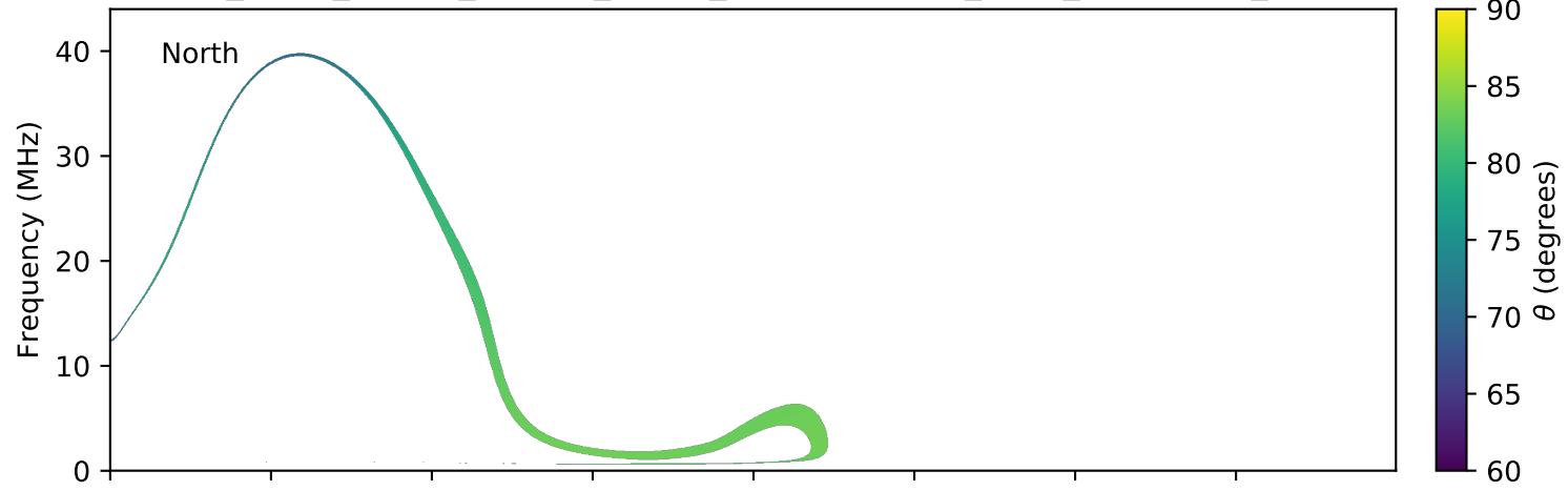
expres_earth_jupiter_europa_jrm09_lossc-wid1deg_3kev_20180415_v01.cdf
