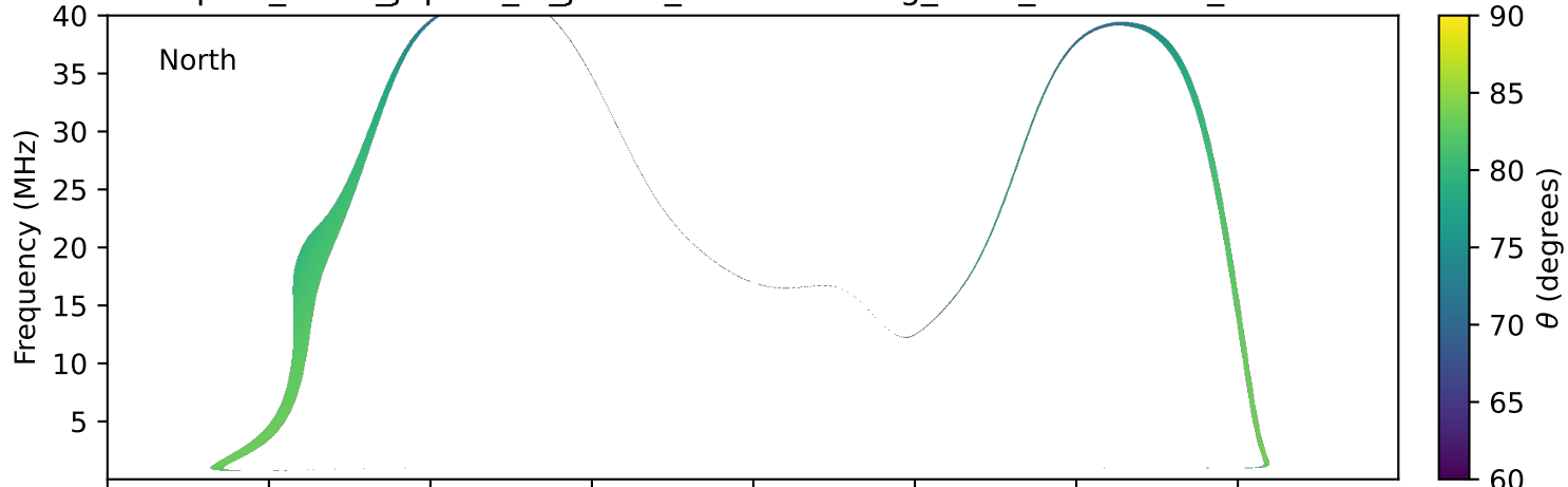
expres_earth_jupiter_io_jrm33_lossc-wid1deg_3kev_20180328_v11.cdf
