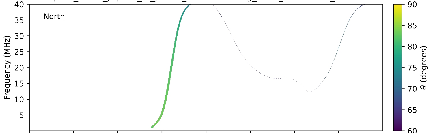
expres_earth_jupiter_io_jrm33_lossc-wid1deg_3kev_20180303_v11.cdf
