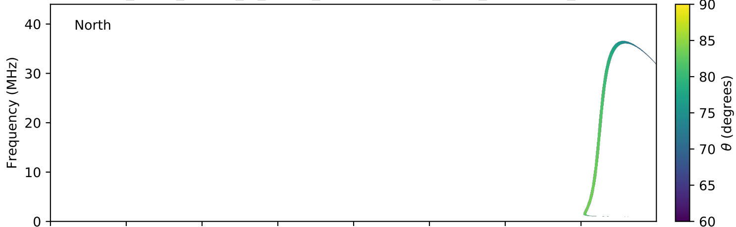
expres_earth_jupiter_io_jrm09_lossc-wid1deg_3kev_20180329_v01.cdf
