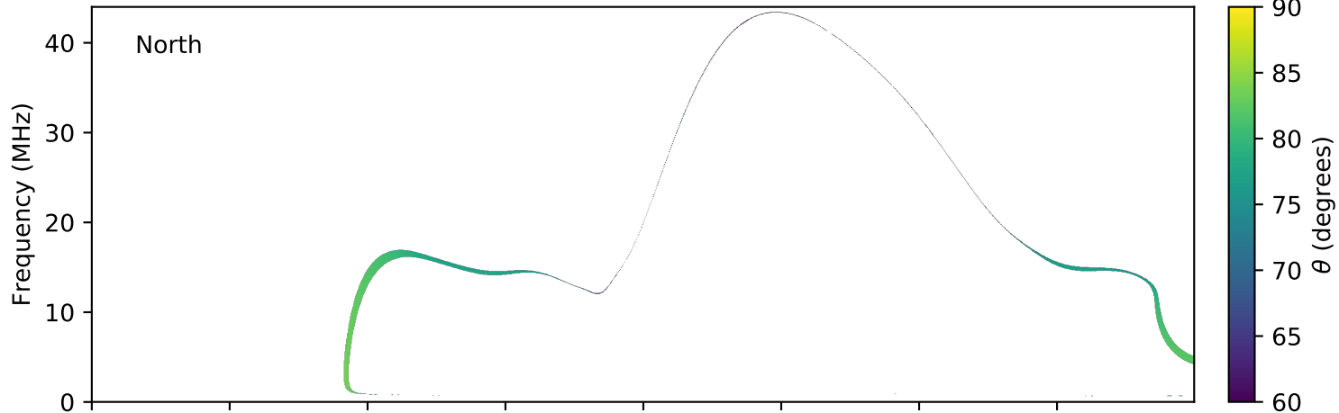
expres_earth_jupiter_io_jrm09_lossc-wid1deg_3kev_20180319_v01.cdf
