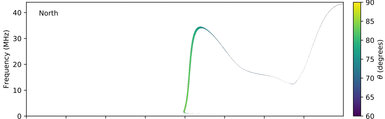
expres_earth_jupiter_io_jrm09_lossc-wid1deg_3kev_20180317_v01.cdf
