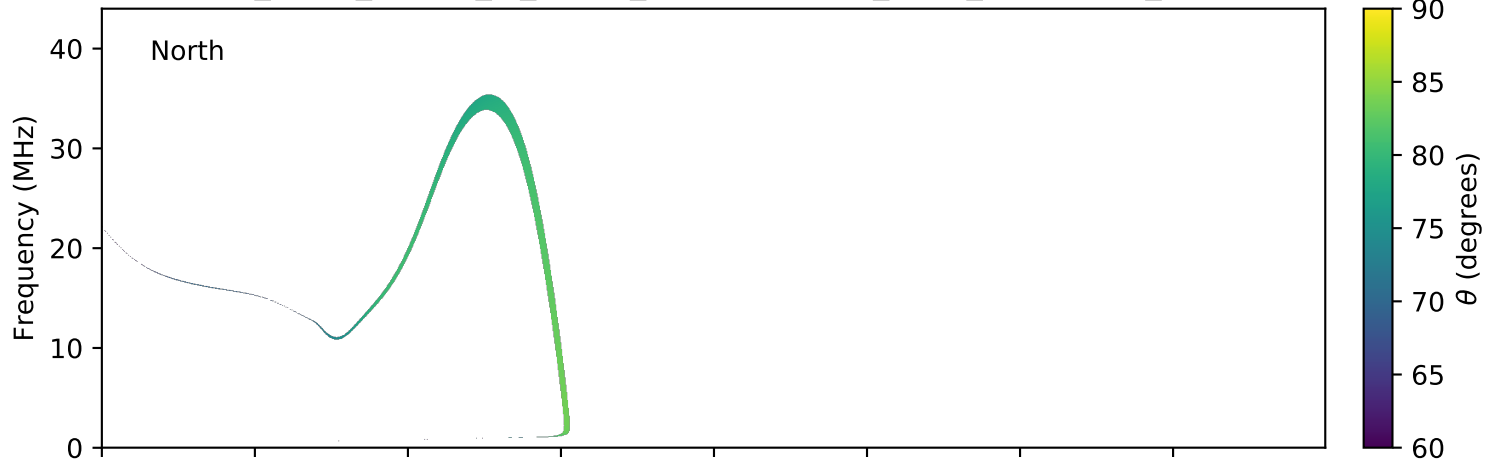
expres_earth_jupiter_io_jrm09_lossc-wid1deg_3kev_20180302_v01.cdf
